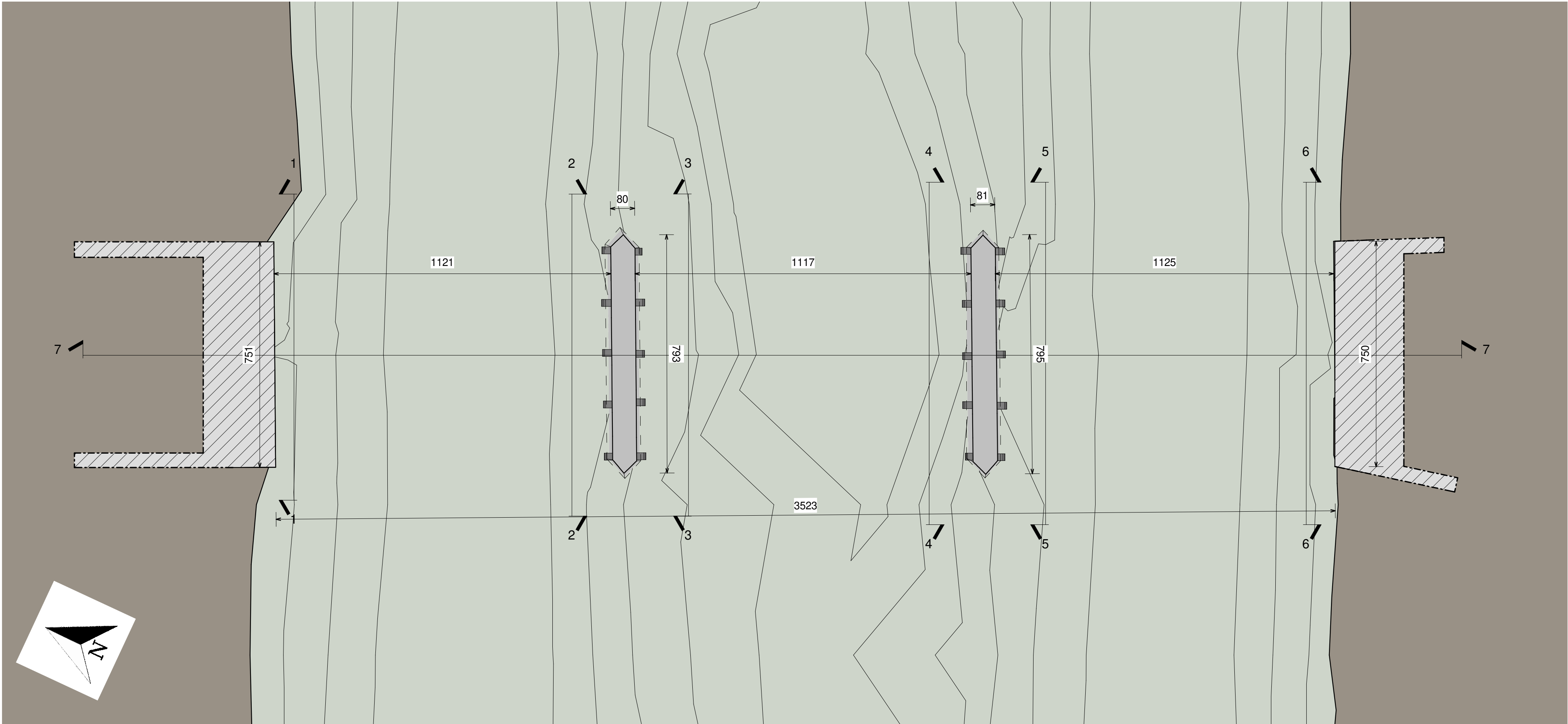
Planimetria Pile
