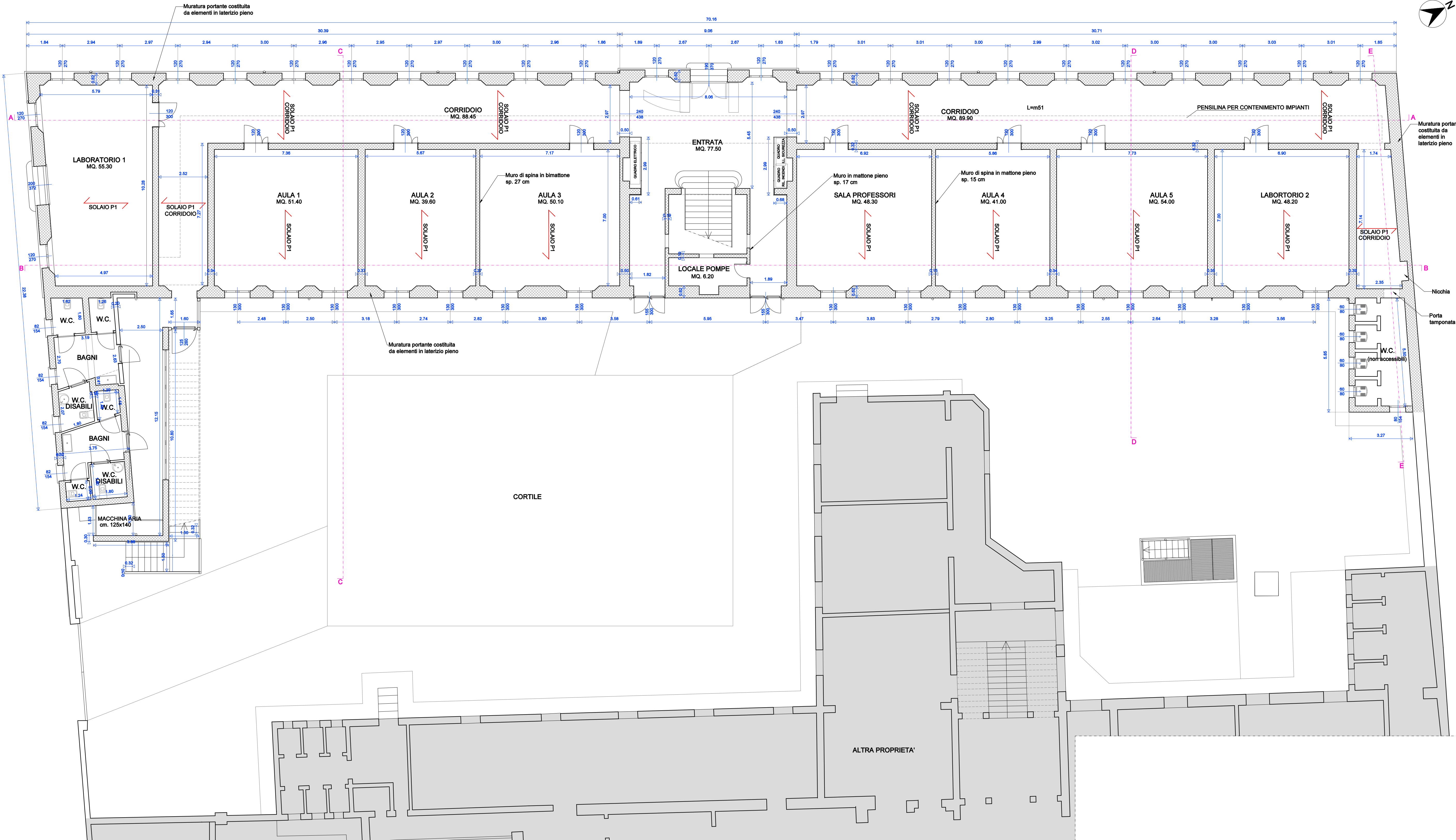
PIANO TERRA
