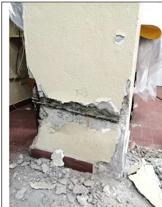
T03 – staffa pilastro
